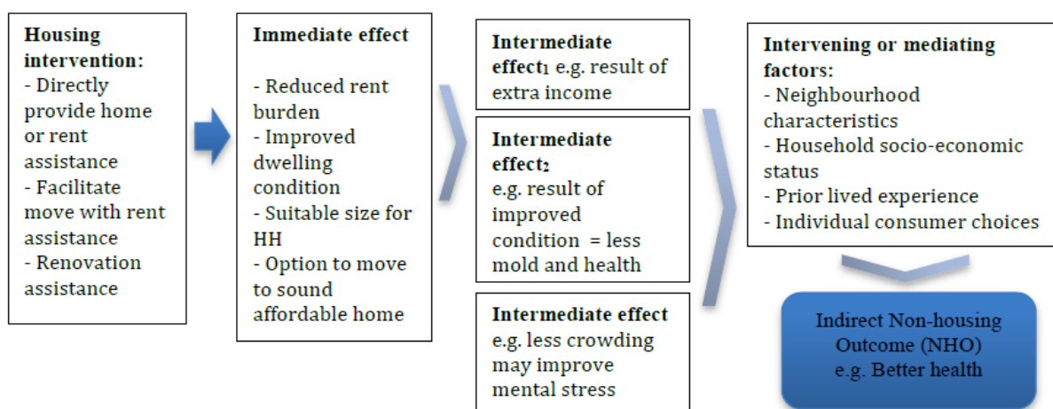
Figure 6.2.3: Causality Chain
