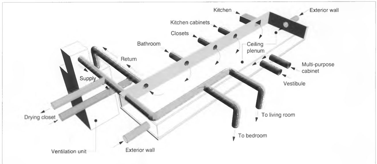
Figure 7: Ventilation Air — Distribution and Returns
