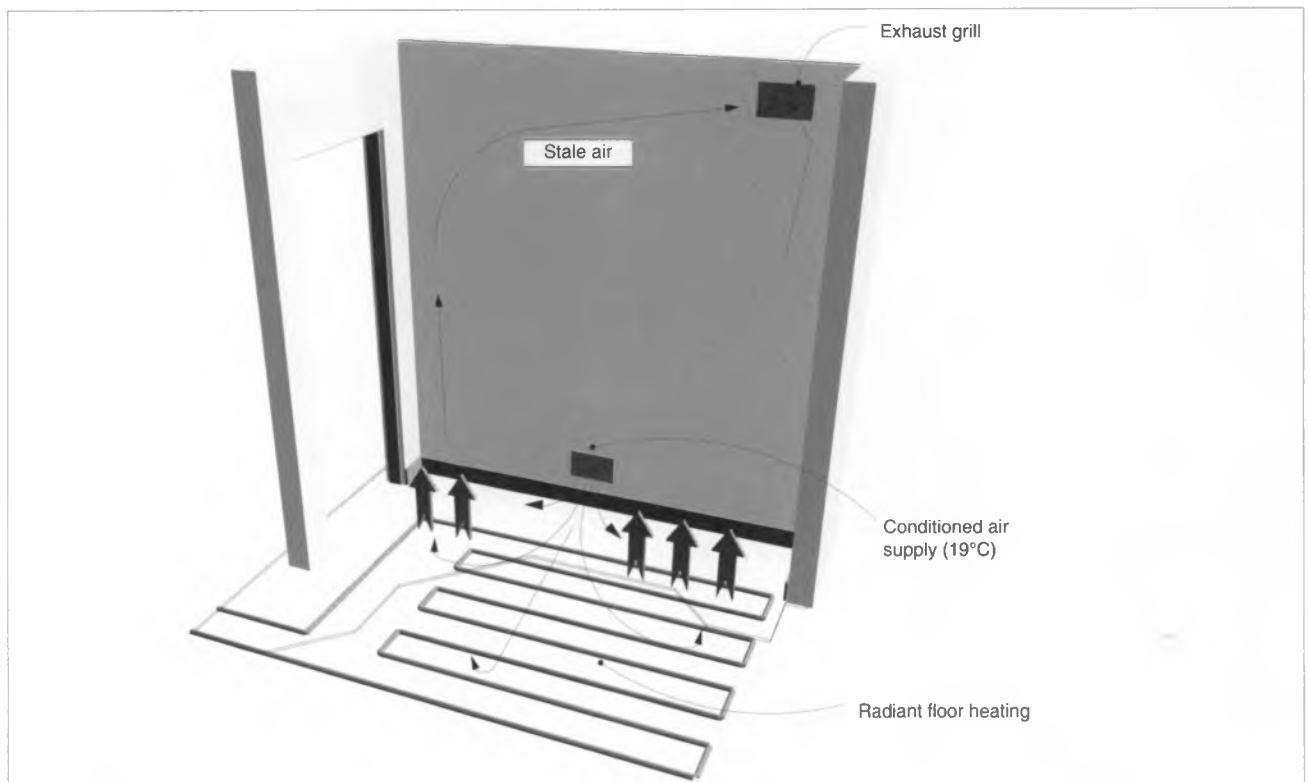
Figure 8: Stratified Ventilation in Bedroom and Living Room
