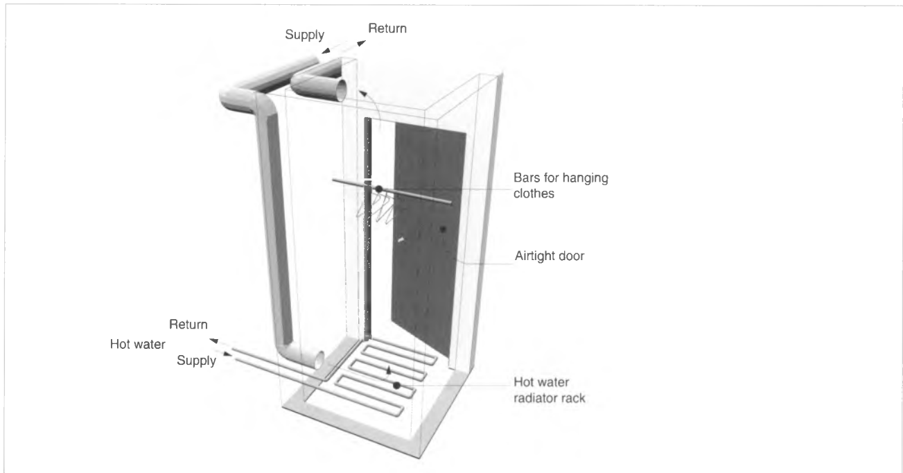
Figure 9: Clothes Drying Closet
