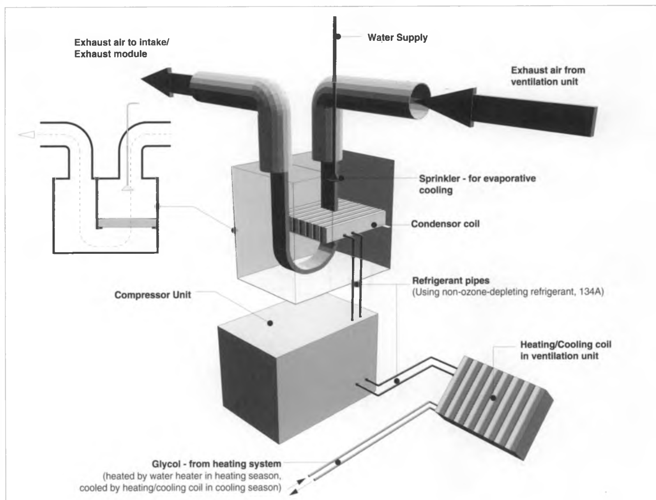
Figure 11: Cooling/Dehumidification System
