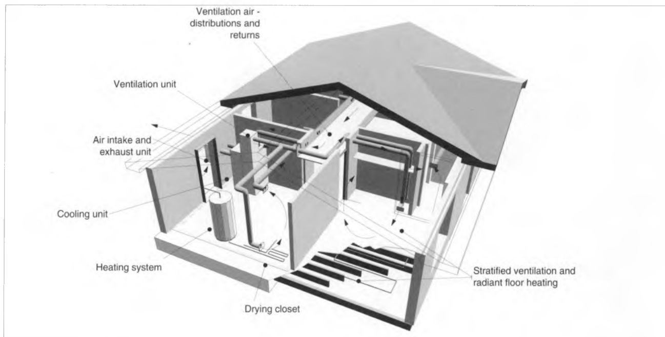
Figure 4: Ventilation System Layout
