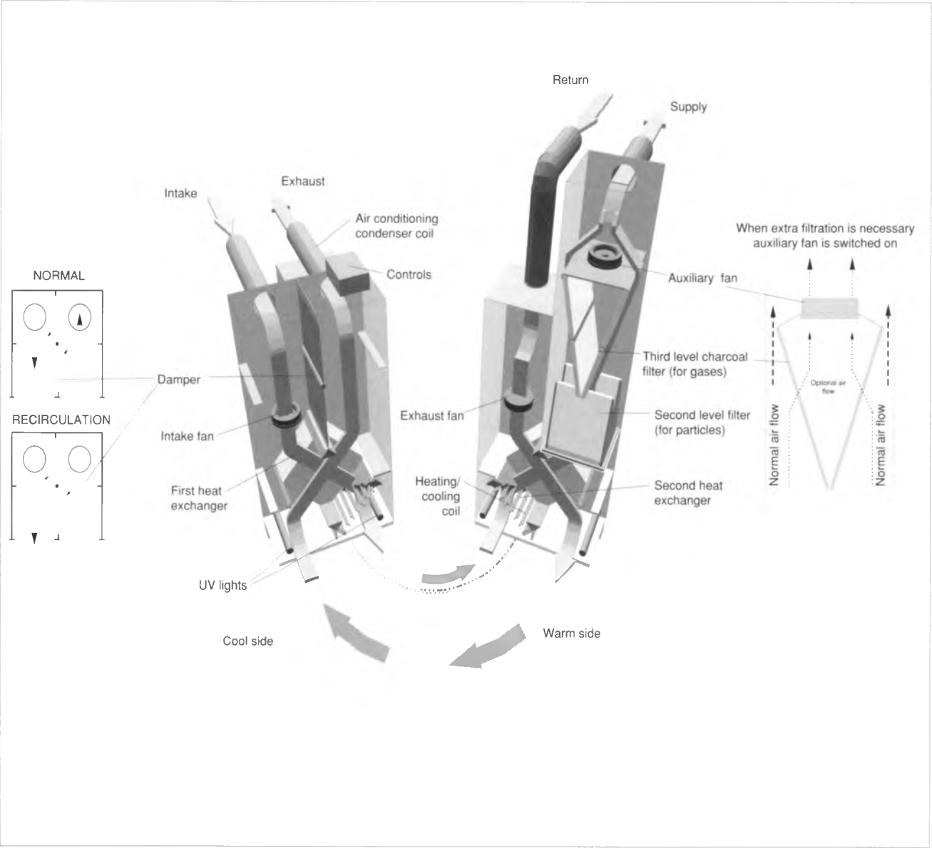
Figure 6: Ventilation Unit
