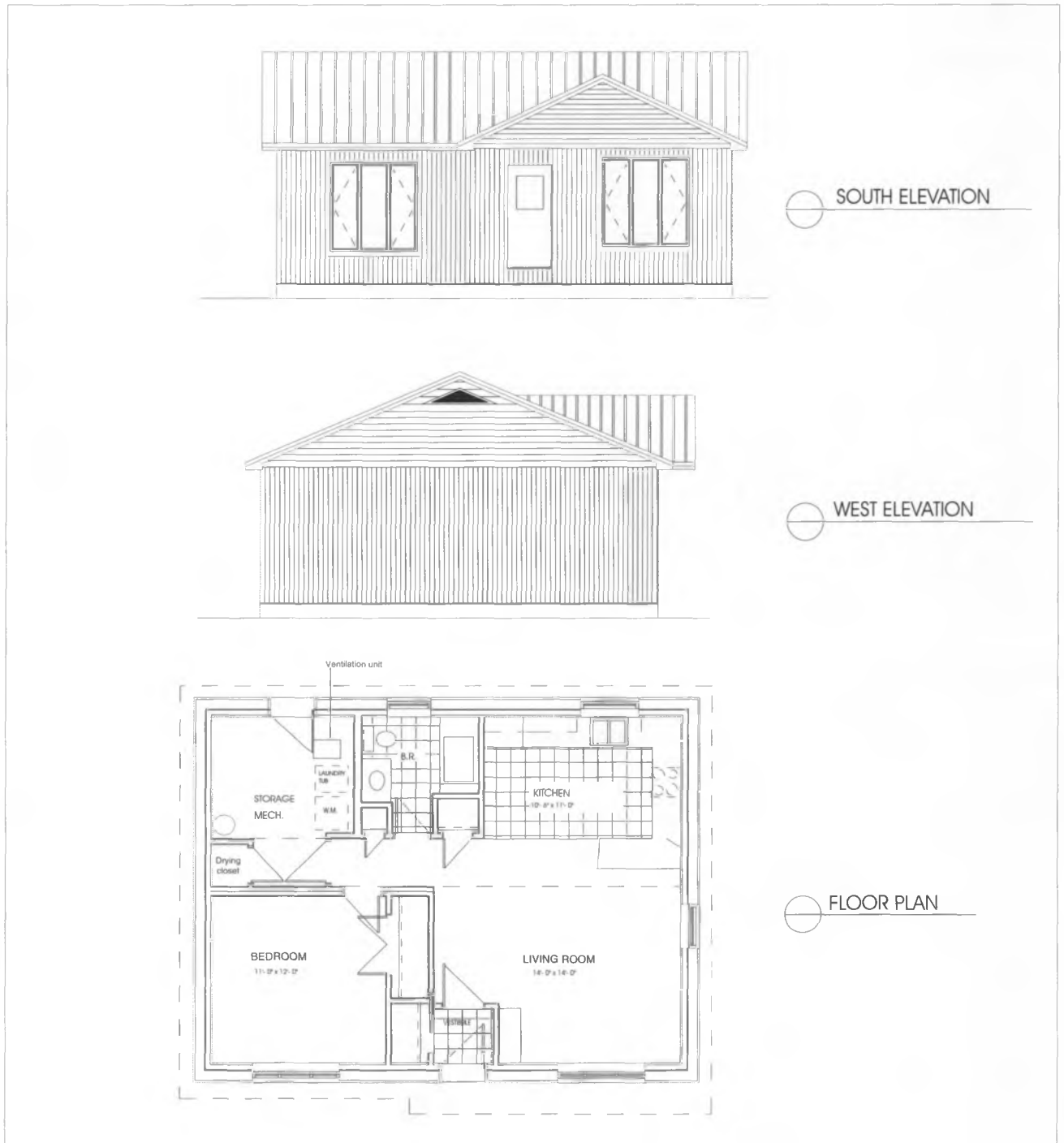
Figure 1: Elevations and Plan of the House
