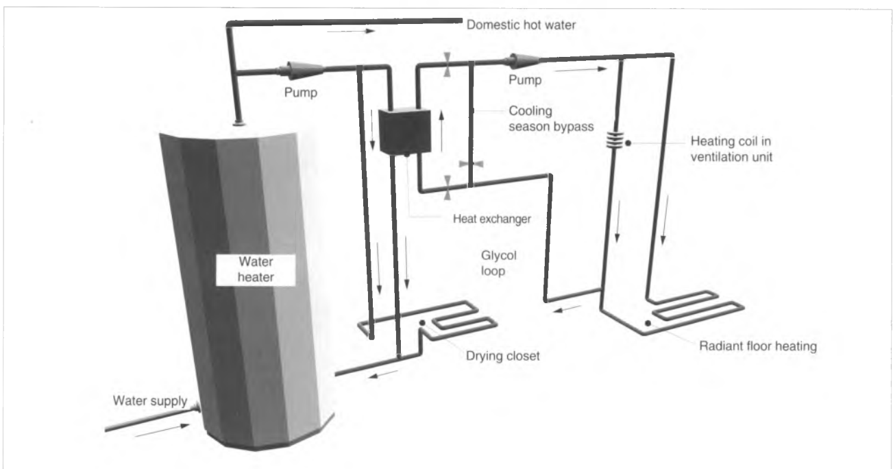
Figure 10: Heating System
