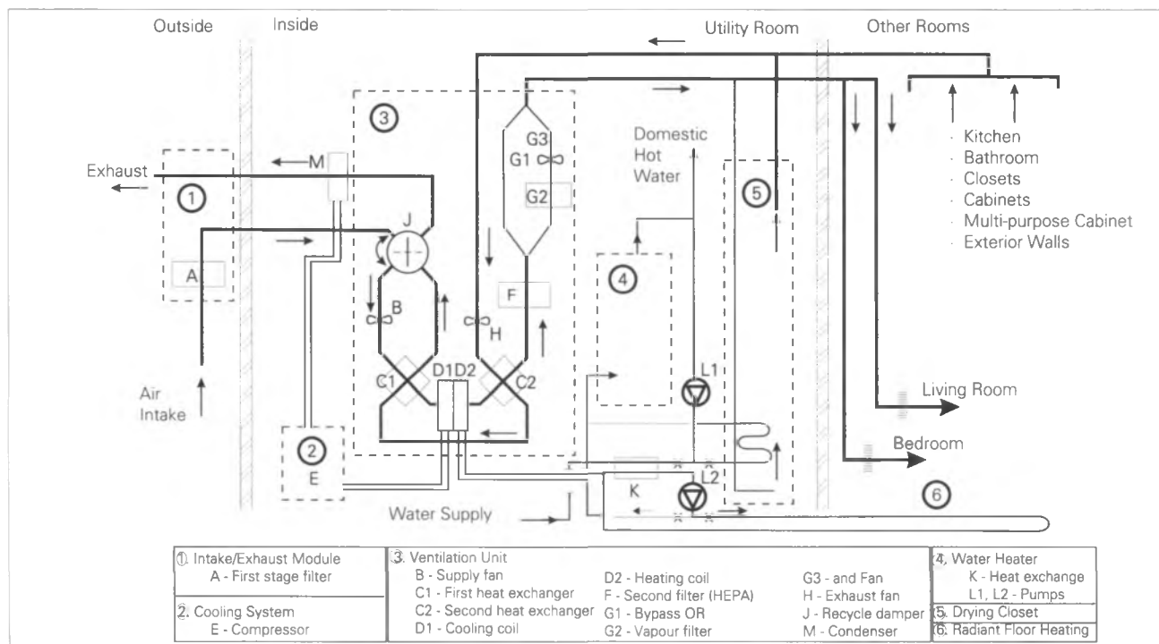
Figure 3: Ventilation System Schematic
