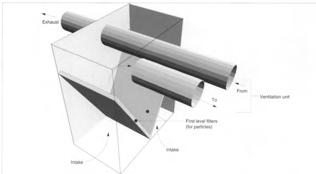
Figure 5: Air Intake and Exhaust Unit (Located Outside)
