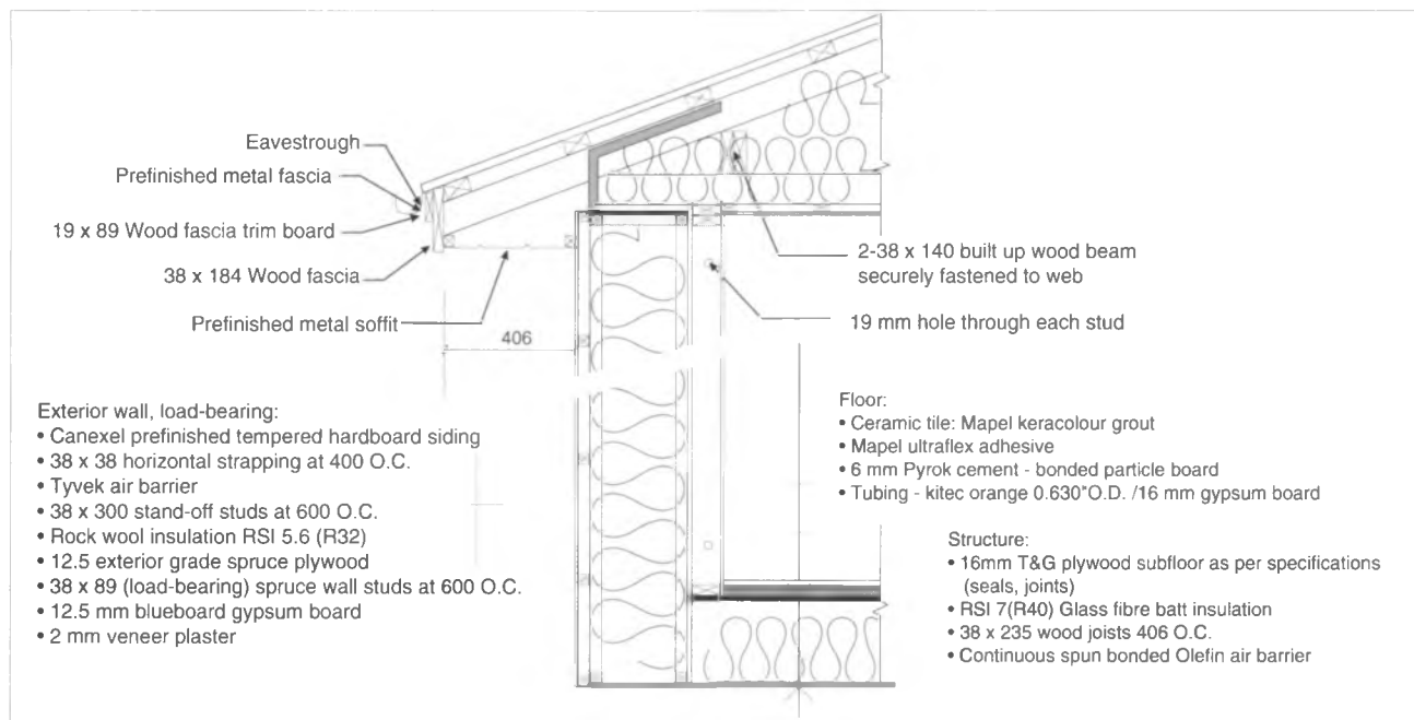
Figure 2: Wall, Roof and Floor Sections
