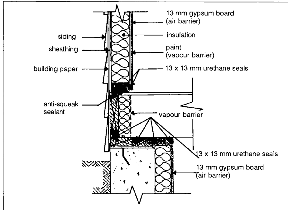
Fig. 6 . Wall/floor/foundation air-barrier detail
