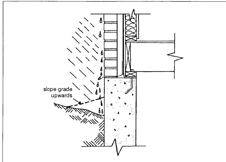
Fig. 22. Water entry into basement area
