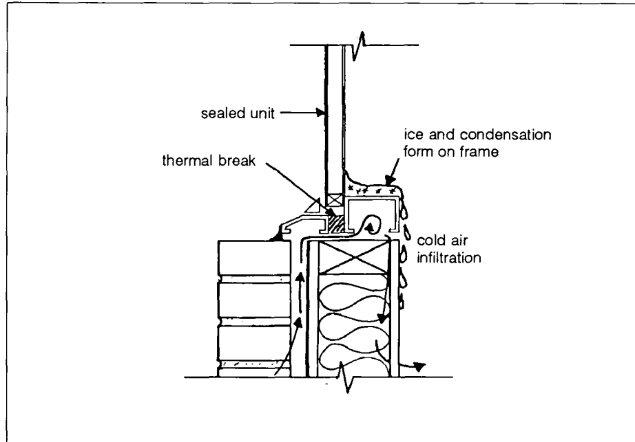
Fig. 34. Window frame not air-sealed to wall
