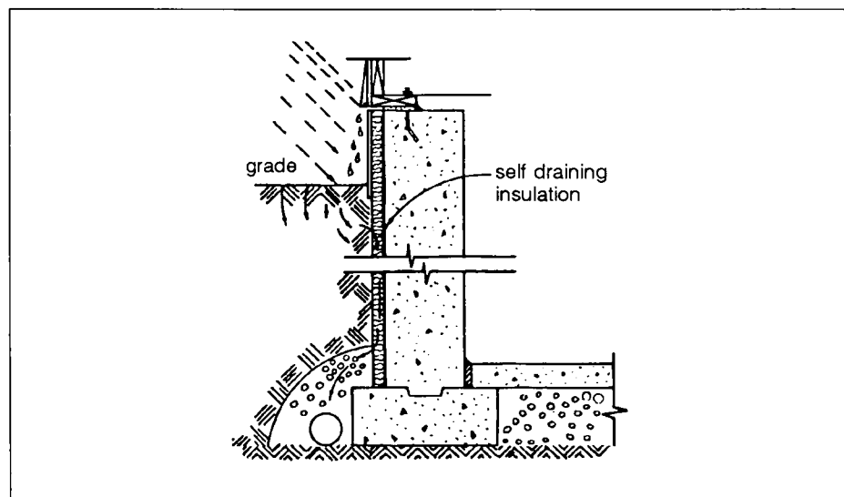
Fig. 2. Basement / foundation-wall drainage detail
