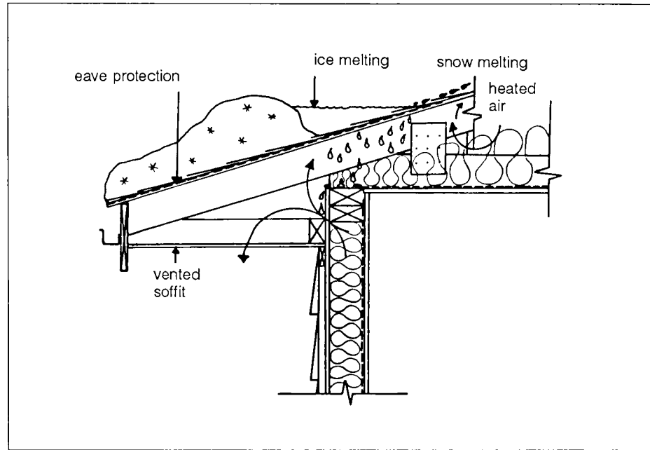
Fig. 18 . Ice damming at edge of roof
