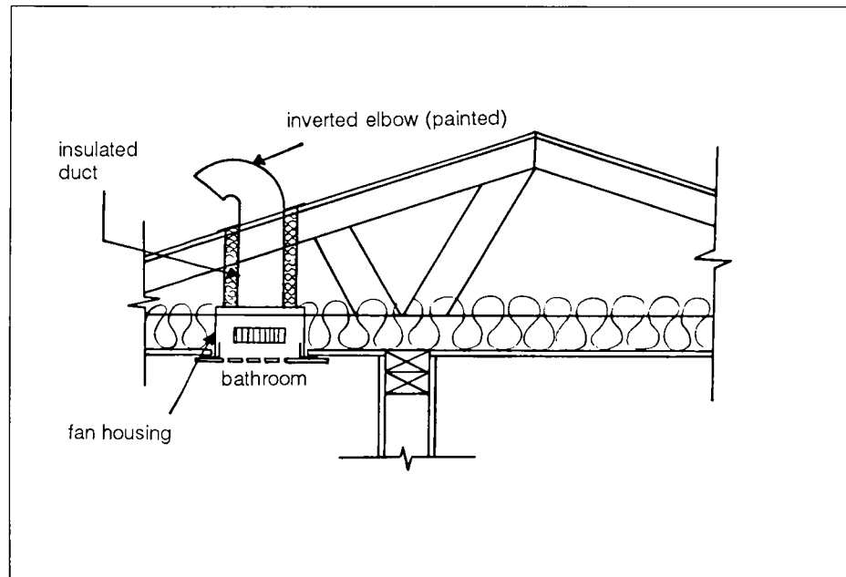
Fig. 19. Bathroom fan / duct installation detail
