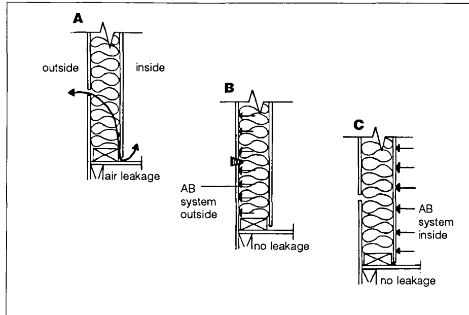
Fig. 3. Location of air barrier in wall
