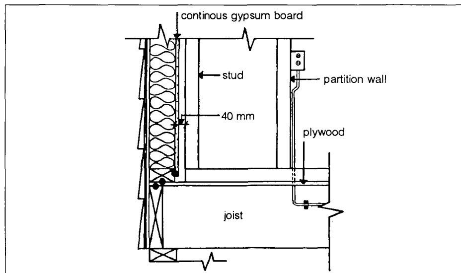
Fig. 9. Exterior wall/partition wall air-barrier detail
