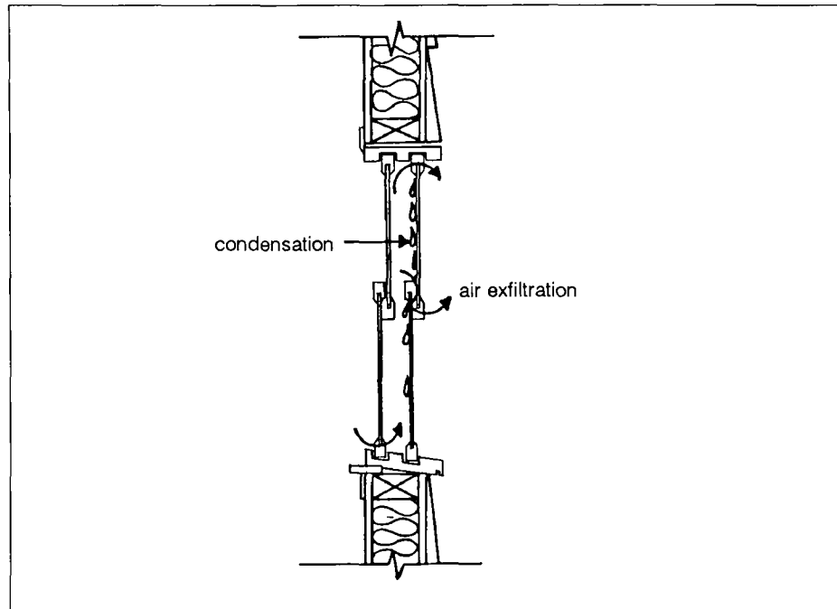
Fig. 32. Condensation of humidity between window panes
