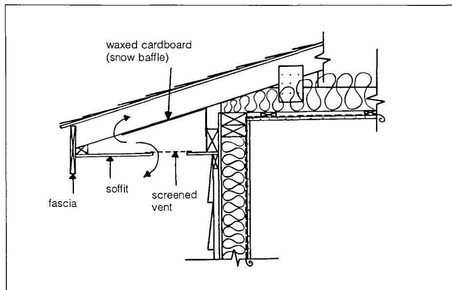
Fig. 17. Soffit baffle prevents entry of blowing snow
