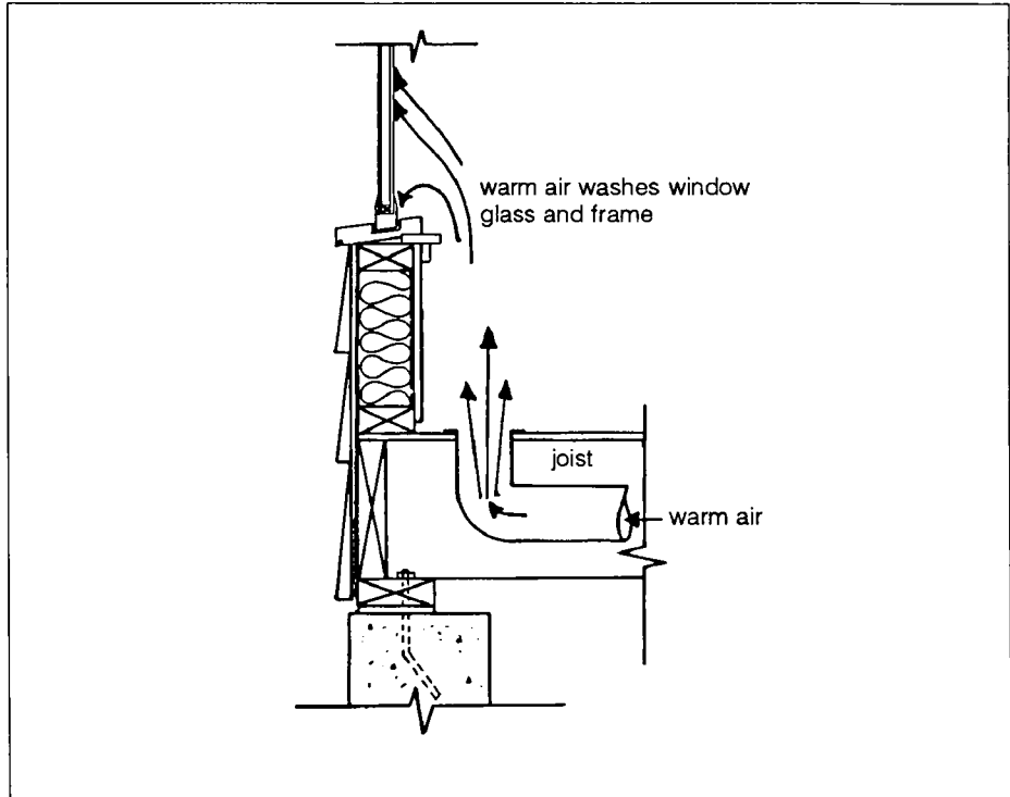
Fig. 35. Circulation of warm air
