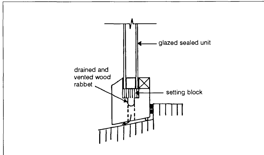
Fig. 36. Lower glazing – sash wood window
