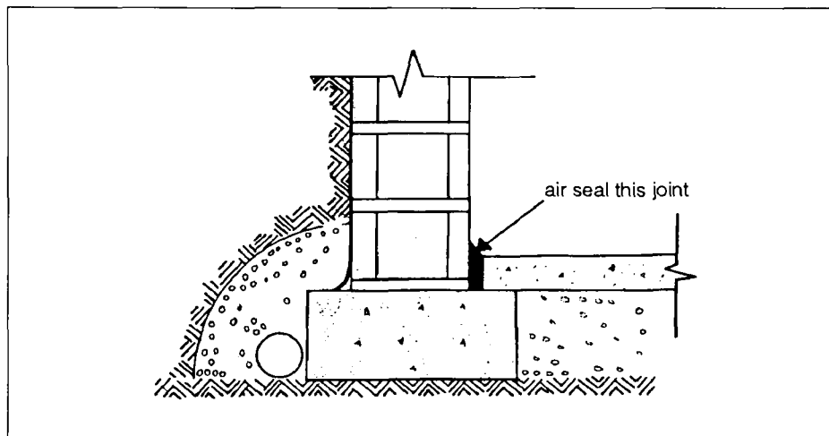
Fig. 24. Air leaks into basement
