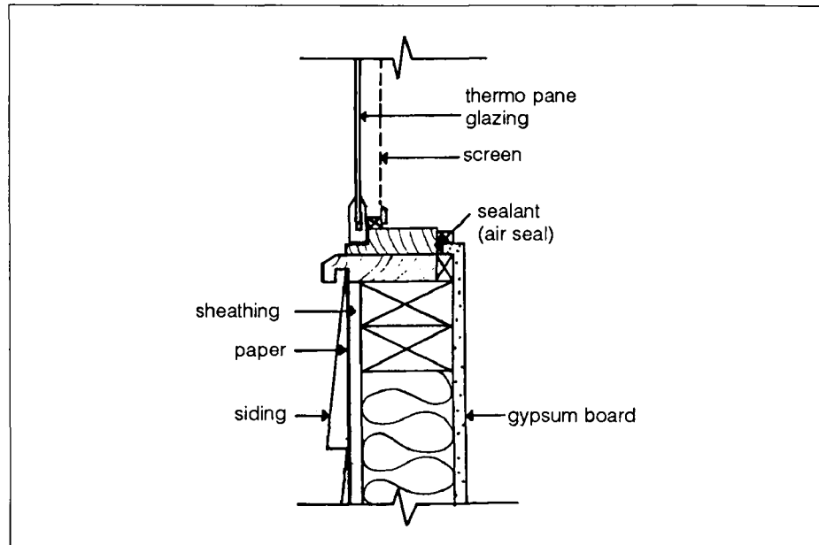
Fig. 10 . Window frame / wall air-barrier detail
