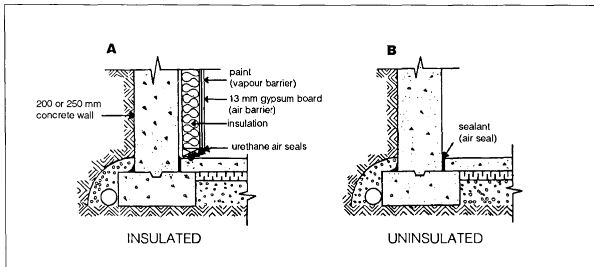
Fig. 5 . Foundation wall/floor air-barrier detail
