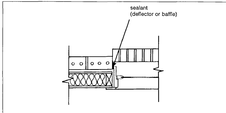
Fig. 28. Direct entry of rain stopped with deflector seal or brick-stop baffle
