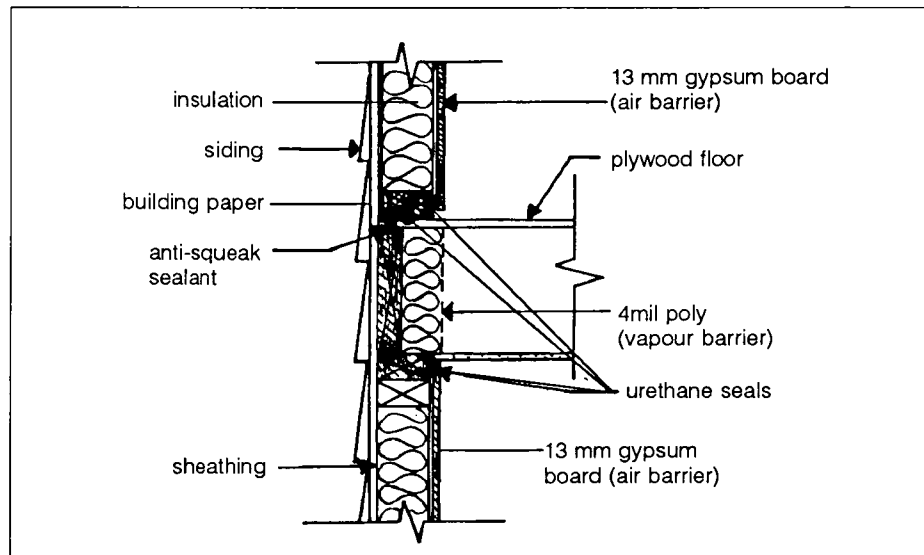
Fig. 7 Exterior wall: second floor air-barrier detail
