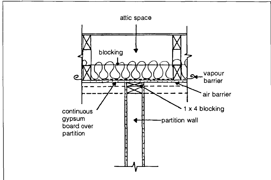
Fig. 8. Partition wall / ceiling air-barrier detail
