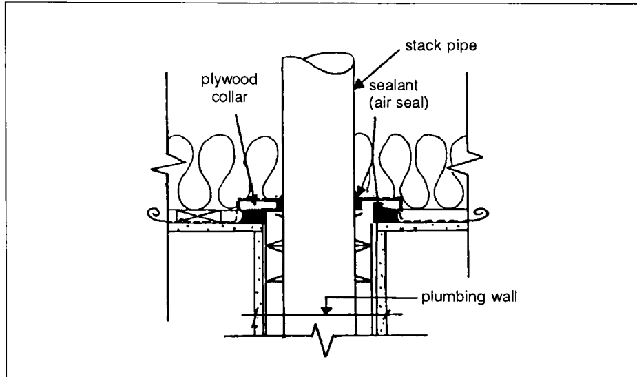
Fig. 12. Stack pipe air-barrier detail
