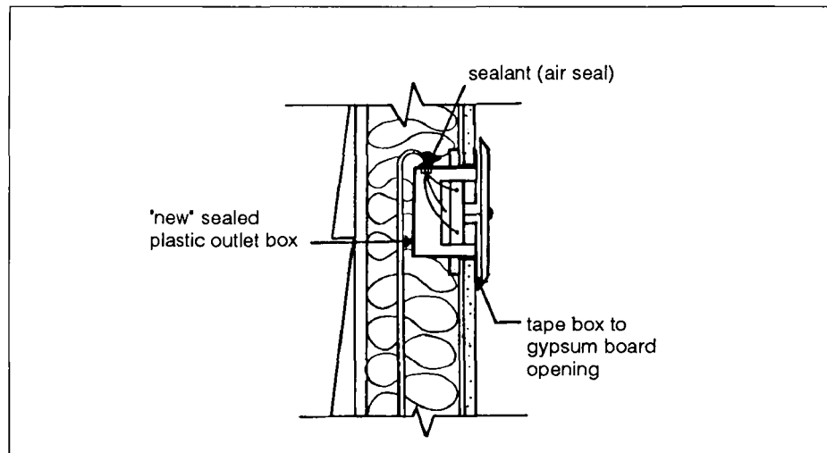
Fig. 11. Air-sealing electrical outlets
