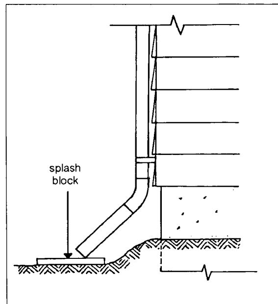
Fig. 23. Drain eavestrough away from house
