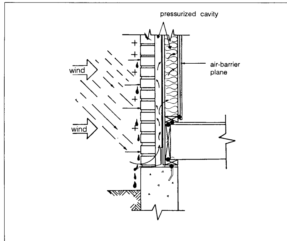
Fig. 13. The rain-screen wall
