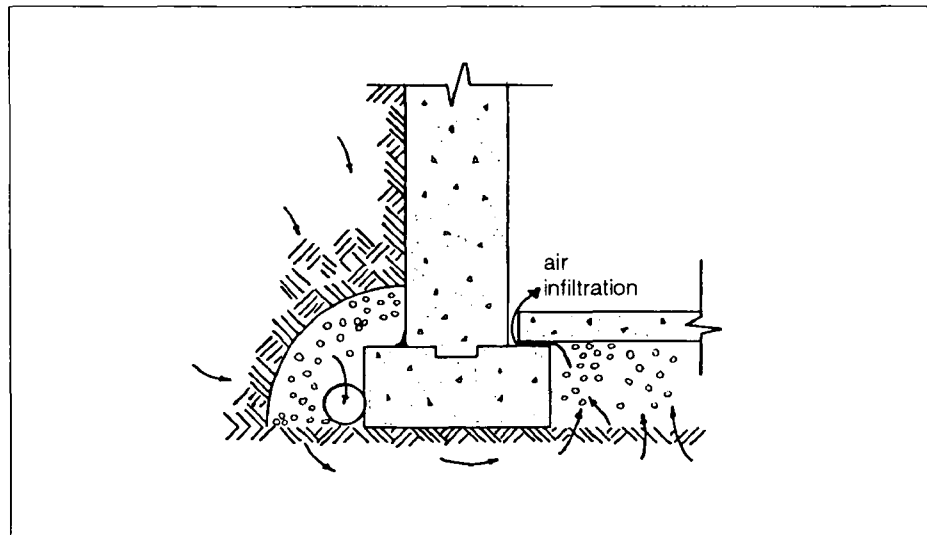
Fig. 21. Air infiltration at foundation / floor joint
