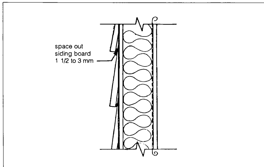
Fig. 20. Wetting of wall by capillary action
