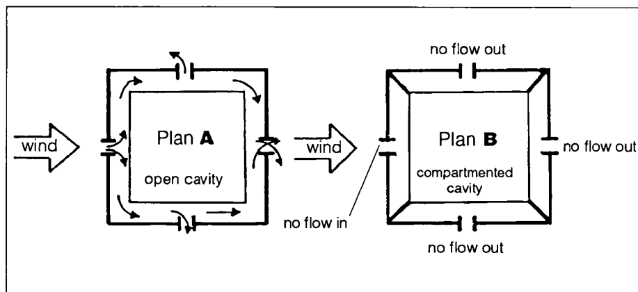
Fig. 14. Open and compartmentalized cavities
