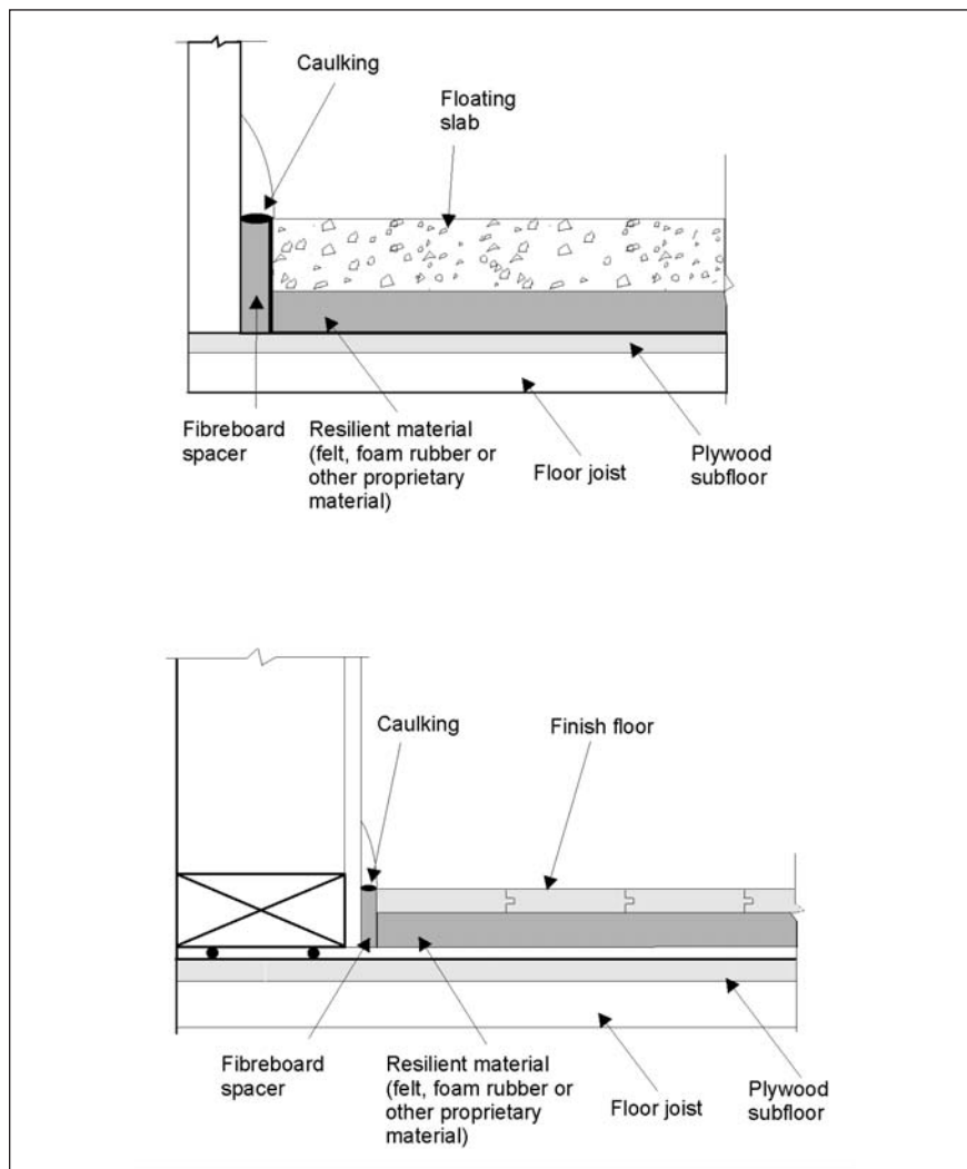
Figure 5.8: Floating floors
