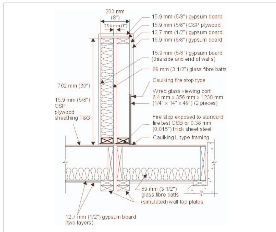
Figure 5.4: Test assembly for fire stop research
